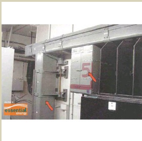
Fuse Cabinets and Busbar Trunking 2.jpg
